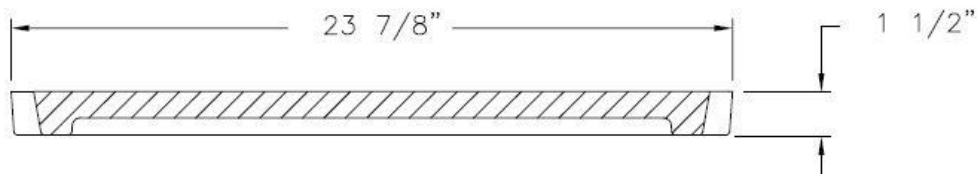
COVER SECTION
